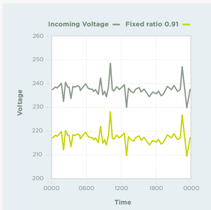
Fixed ratio transformer
